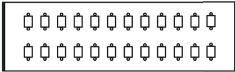
24 LC Duplex or 24 E2000 or 24 SC Simplex Vertical Adaptor Plate
